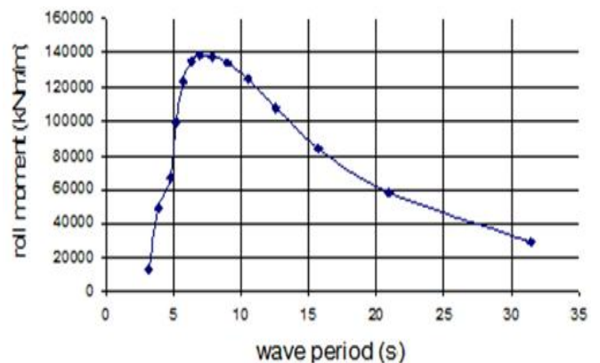
Figure 6: Variation of roll moment with wave period
