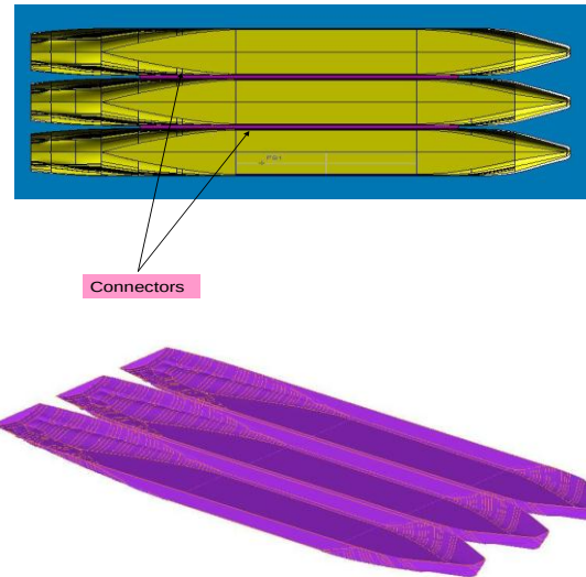
Figure 2: Geometry of the carrier vessel - Bottom view & isometric view
