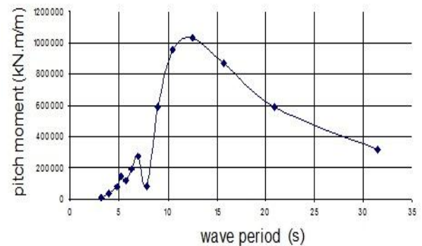
Figure 17: Variation of pitch moment with wave period
