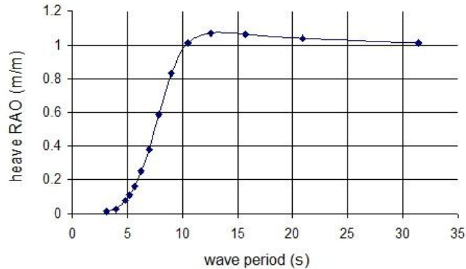
Figure 19: variation of heave response with wave period
