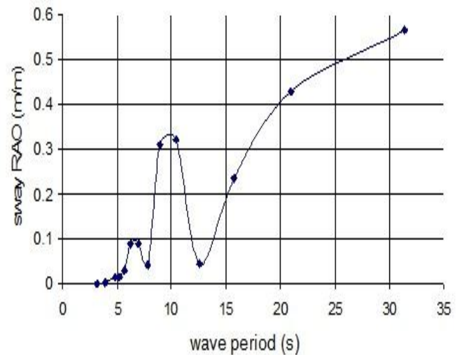
Figure 23: variation of sway response with wave period
